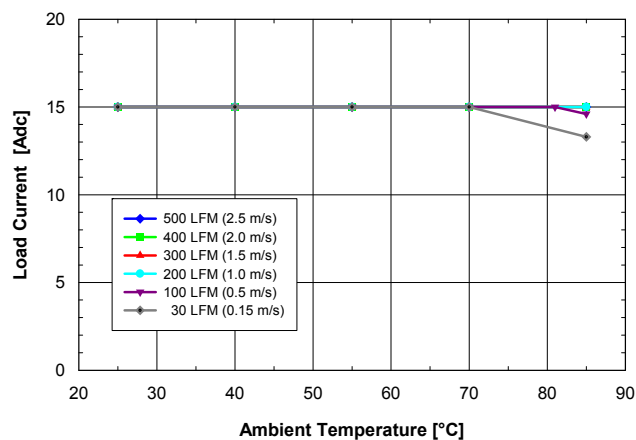
Fig. 1.5V.2: Available load current vs. ambient air temperature and airflow rates for SQ48T15015 converter with D height pins mounted horizontally with V_{in} = 48\text{ V} , air flowing from pin 3 to pin 1, and maximum FET temperature \leq 120\text{ }^\circ\text{C} .
