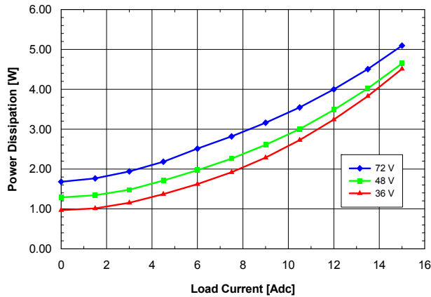
Fig. 2.0V.7: Power dissipation vs. load current and input voltage for SQ48T/S15020 converter mounted vertically with air flowing from pin 3 to pin 1 at a rate of 300 LFM (1.5 m/s) and T_a = 25\text{ }^\circ\text{C} .
