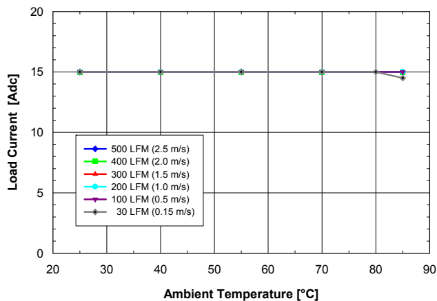
Fig. 1.0V.2: Available load current vs. ambient air temperature and airflow rates for SQ48T15010 converter with D height pins mounted horizontally with V_{in} = 48\text{ V} , air flowing from pin 3 to pin 1, and maximum FET temperature \leq 120\text{ }^\circ\text{C} .
